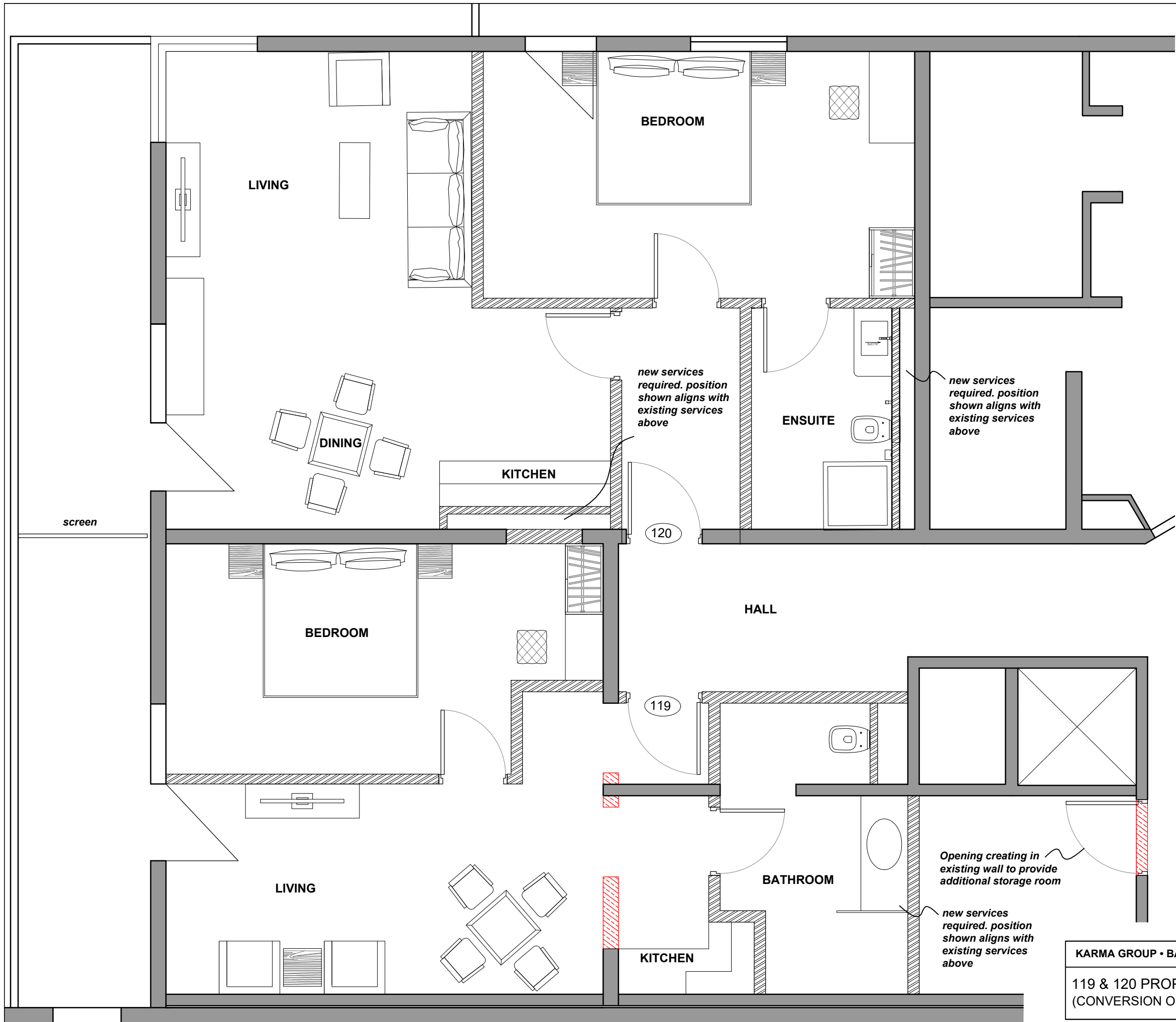
PROPOSED PLAN @ 1:50
